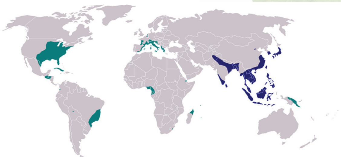
Figure 8: Distribution of Aedes albopictus as of December 2007 CDC 128
