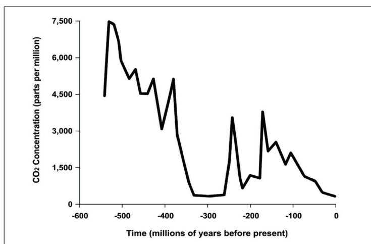
Figure 5. CO 2 Levels on Earth: A Long View*
